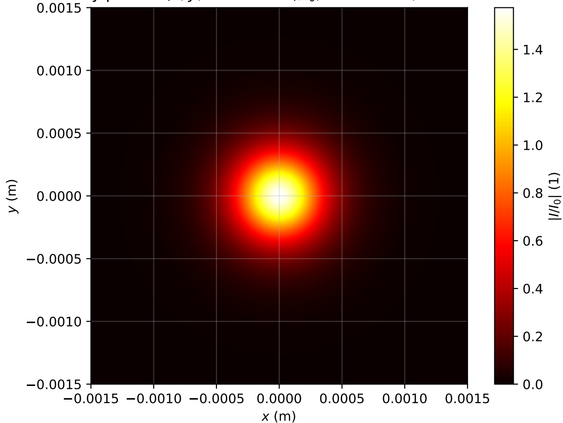
Intensity profile I(x, y, z = 2.946m)/I_0 , P_{in}=0.9P_{cr} , artificial time
